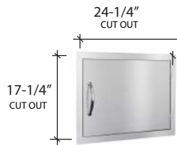
BBQ-DRSS-2418 ACCESS DOOR stainless steel
