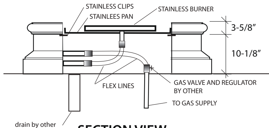
SECTION VIEW
