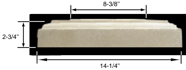
PC-221-14 Side View
