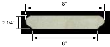
WC-720-6 Side View
