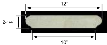
WC-720-10 Side View
