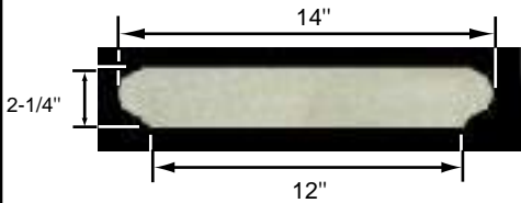
WC-720-12 Side View
