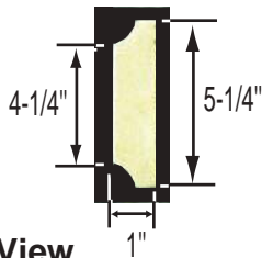
Side View MD-525
