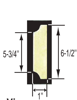
Side View MD-6530S
