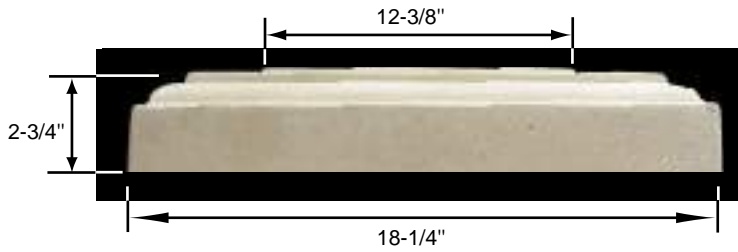
PC-221-18 Side View
