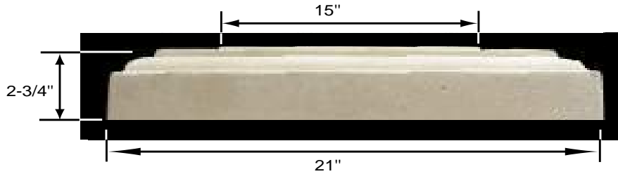
PC-221-21 Side View
